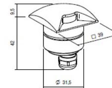
C.C. version
