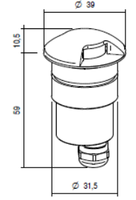
24Vdc version
