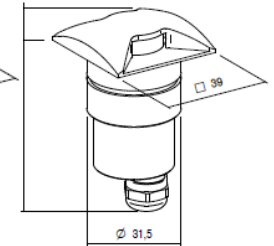
24Vdc version
