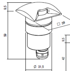
24Vdc version
