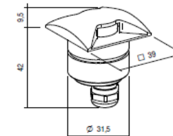
C.C. version
